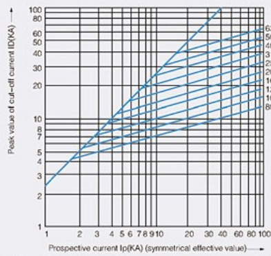
'RO201~203' Characteristic curve of cut-off current of 'gG' fuse link
