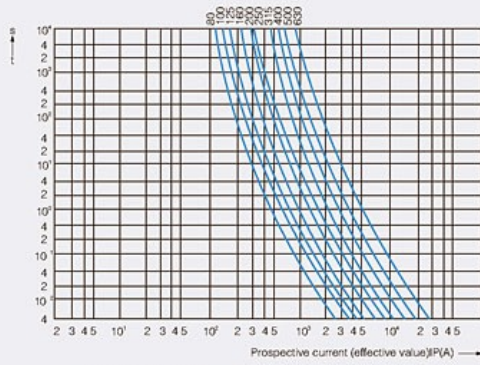
'RO201~203' Time-current band of 'gG' fuse link
